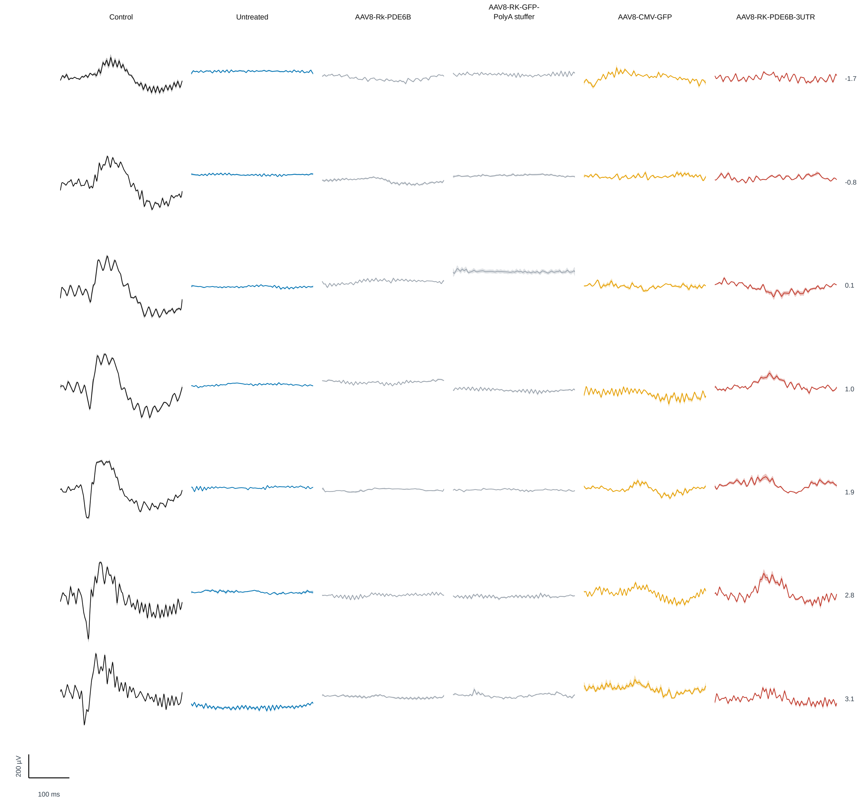
Mean scotopic ERG ( \pm SEM, n=5)
